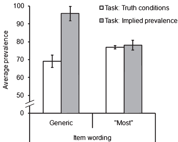
Fig. 2. The average prevalence that led participants in Experiment 1 to accept statements (the truth conditions task, white bars) versus the average prevalence implied by the same statements (the implied prevalence task, gray bars). The error bars represent \pm 1 SEM.
